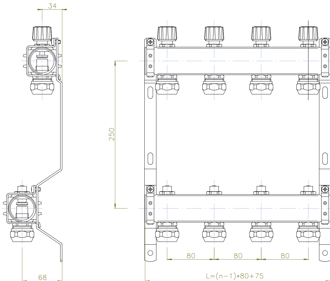
L = Length of manifold n = Number of circuits
