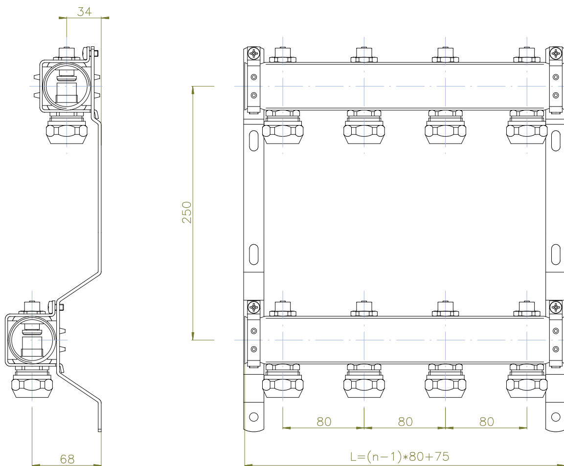
L = Length of manifold n = Number of circuits
